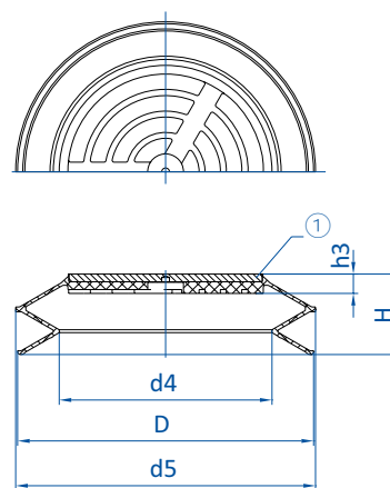
Drawing B
