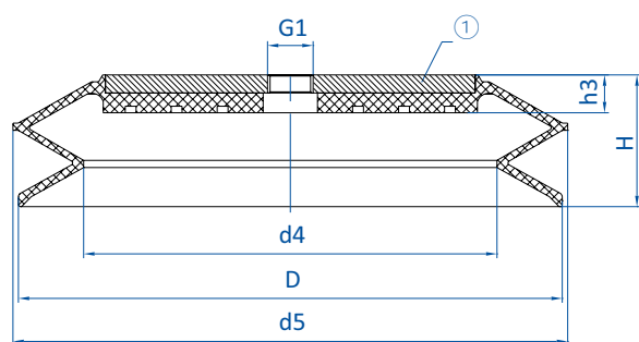
Drawing A
